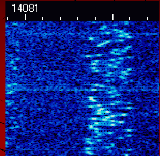
MFSK Trace
