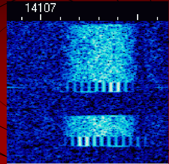
HF Packet Trace
