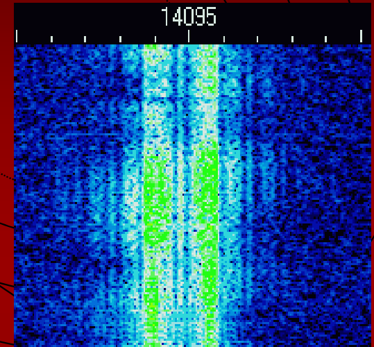
AMTOR Trace
